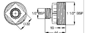
BRASS 1/2" BSP x 1 1/2" BSP AIR GAP COUPLING
