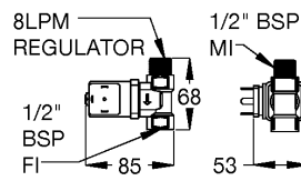
STAINLESS STEEL SOLENOID VALVE
